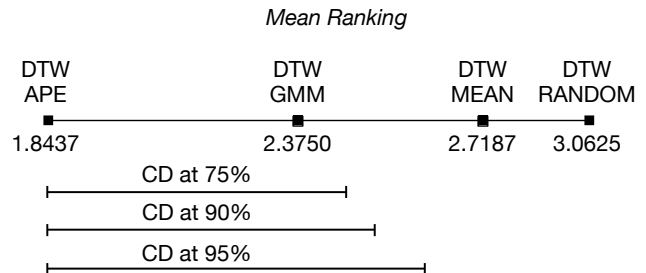
Fig. 9. Mean rank per method and critical difference interval for difference confidence values.
