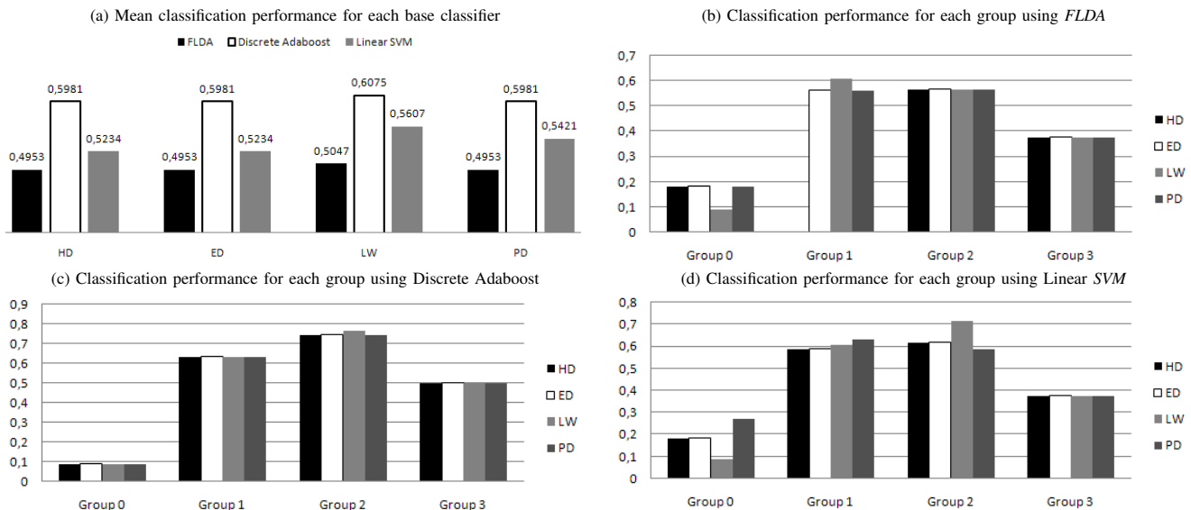
Fig. 4. Leave-one-patient-out classification using one-versus-one ECOC design (HD: Hamming decoding, ED: Euclidean decoding, LW: Loss-Weighted decoding, PD: Probabilistic decoding) for the four groups with and without Chagas' disease.
