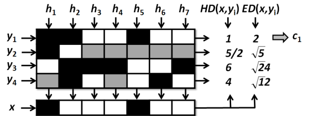
Fig. 1. Example of ternary matrix M for a 4-class problem. A new test codeword is classified by class c_1 when using the traditional Hamming and Euclidean decoding strategies.
