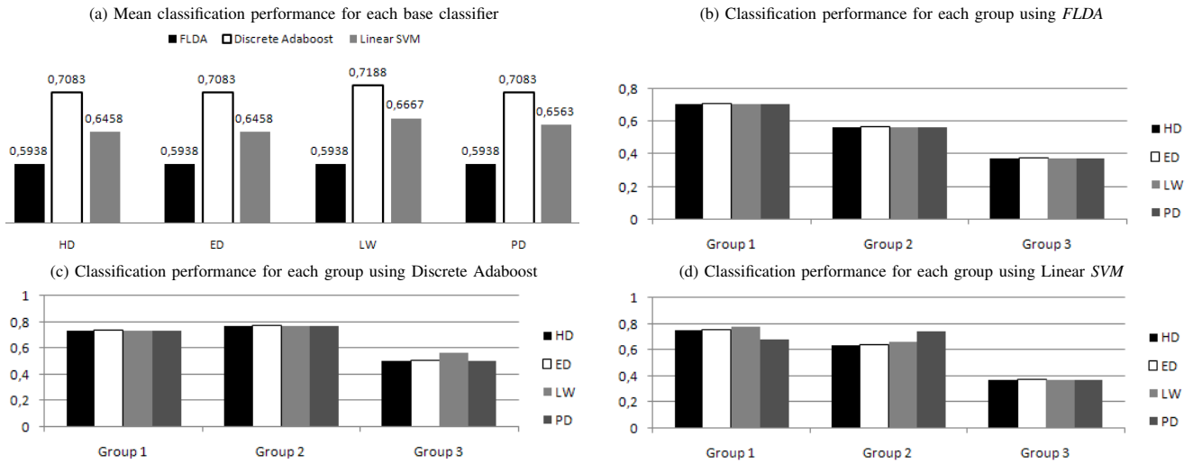
Fig. 5. Leave-one-patient-out classification using one-versus-one ECOC design (HD: Hamming decoding, ED: Euclidean decoding, LW: Loss-Weighted decoding, PD: Probabilistic decoding) for the three groups with Chagas' disease.
