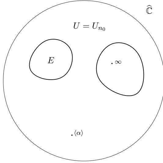
Figure 18: U is a multiply-connected subset of \mathcal{A}^* such that f(U) is simply connected. If U were unbounded, the point at infinity would be in \partial(\hat{\mathbb{C}} \setminus (U \cup E)) (see Figure 19).
