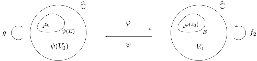
Figure 6: The properties of g (including the existence of a weakly repelling fixed point) are transferred to f_2 due to the conjugacy \phi . Recall that V_0 = \widehat{\mathbb{C}} \setminus E .
