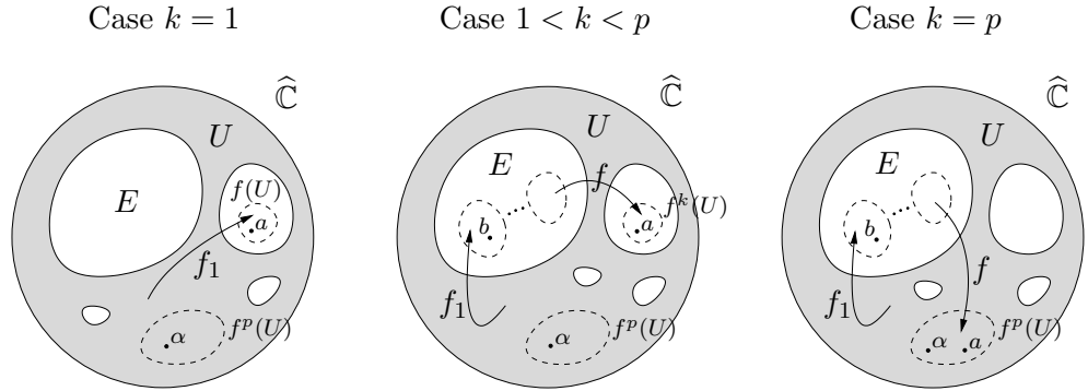
Figure 8: The topological surgery construction for the three possible cases, drawn on \widehat{\mathbb{C}} .
