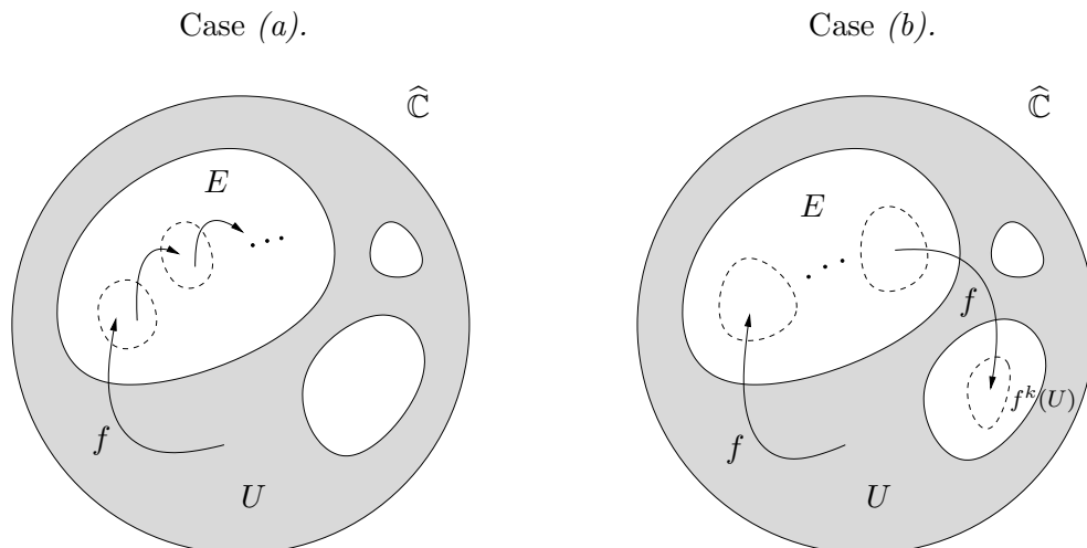
Figure 20: The two possible situations. In (a), the iterations of U always stay in E , f^k(U) \subset E for all k \in \mathbb{N} ; whereas in (b), there exists k \in \mathbb{N} such that f^i(U) \subset E for all 0 < i < k and f^k(U) \subset \widehat{\mathbb{C}} \setminus E .
