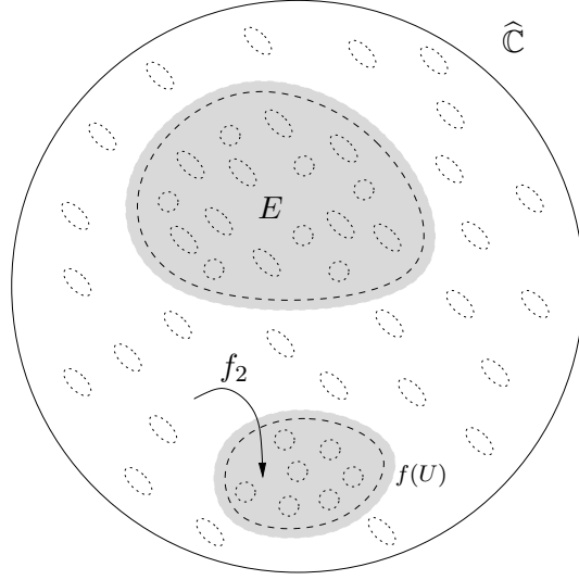
Figure 5: Construction of the almost complex structure \sigma . Recall that U = \widehat{\mathbb{C}} \setminus E . The grey area denotes the region where f_2 is holomorphic.
