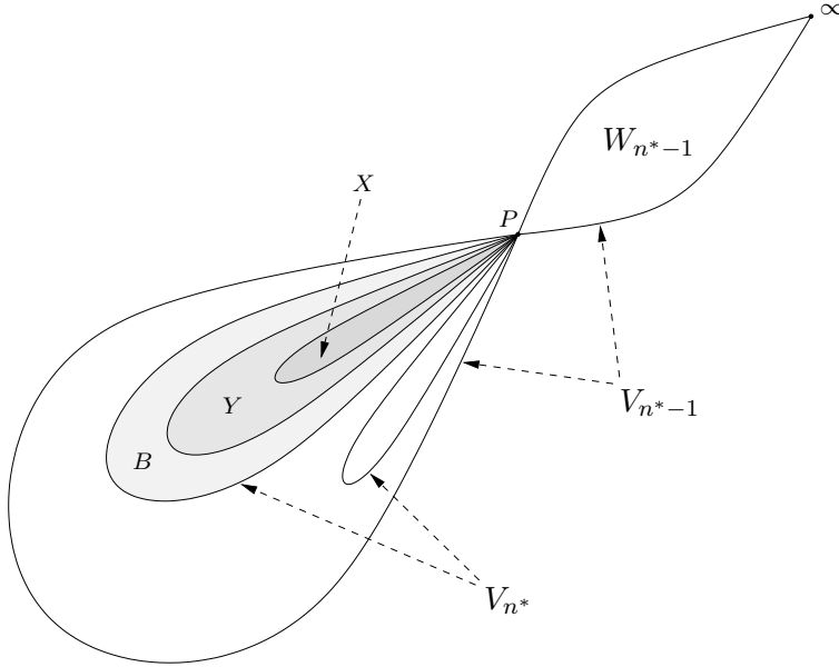
Figure 17: In the situation where X lies in one of the bounded components B of \mathring{V}_{n^*} , there exists a preimage Y of W_{n^*-1} such that X \subset Y \subset B .
