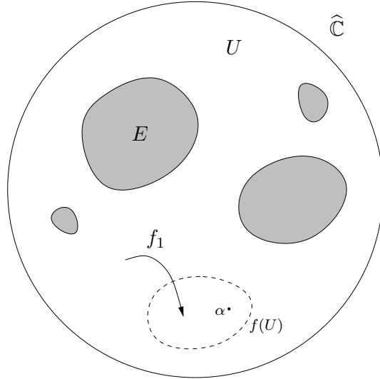
Figure 4: The sets U , f(U) and E on the Riemann sphere. The shaded sets are connected components of \widehat{\mathbb{C}} \setminus U .
