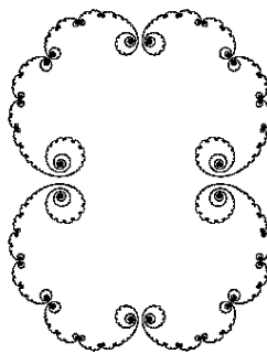
(b) F(z) = z^2 + 0,25
