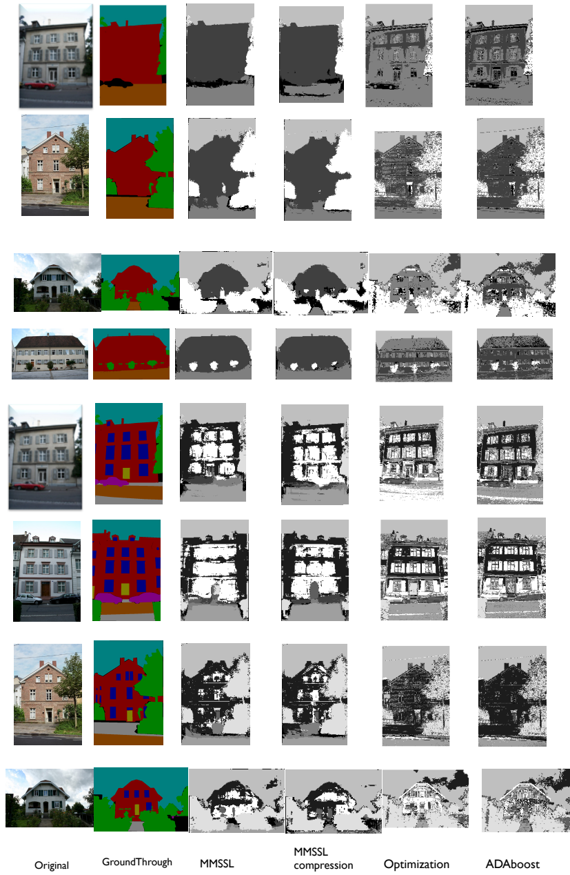
Fig. 5. Etrims 4-class (four top rows) and 8-class (four bottom rows) results
